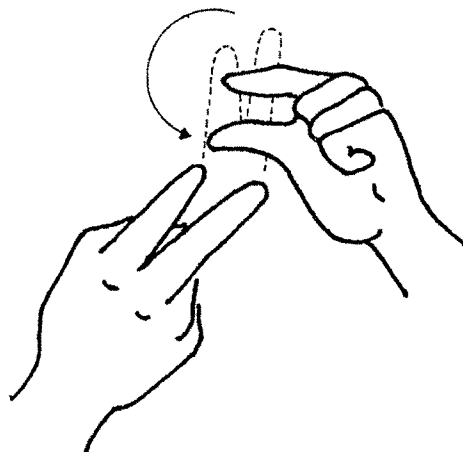
ADVERB
