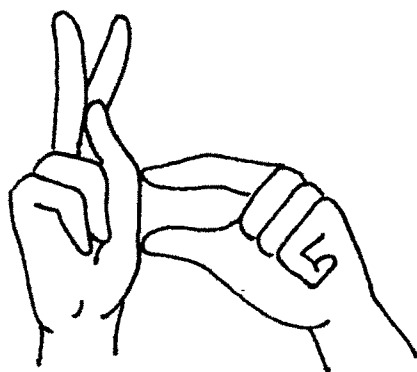
TENSE
