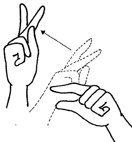
PAST TENSE
