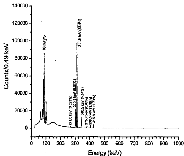
Fig. 1. Gamma-ray spectrum of radiochemically separated ^{233}\text{Pa} showing seven different \gamma -rays with their branching intensities.
