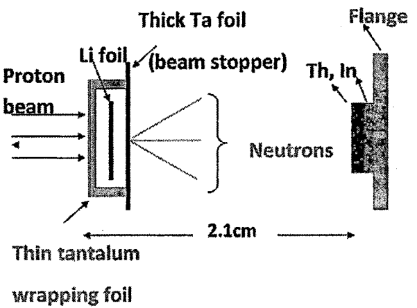
Fig. 1. Schematic diagram showing the arrangement used for the neutron irradiation.
