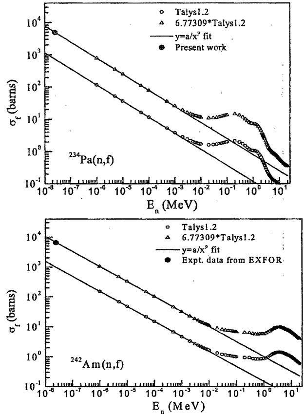
Fig. 3. Plot of experimental and theoretical ^{234}\text{Pa}(n,f) and ^{242}\text{Am}(n,f) cross-section. Theoretical fission cross-sections above 1 keV were calculated using the TALYS computer code version 1.2. The fission cross-section below 1 keV up to thermal energy was extrapolated by a normalized fit of the 1/v formula as shown in the figure.
