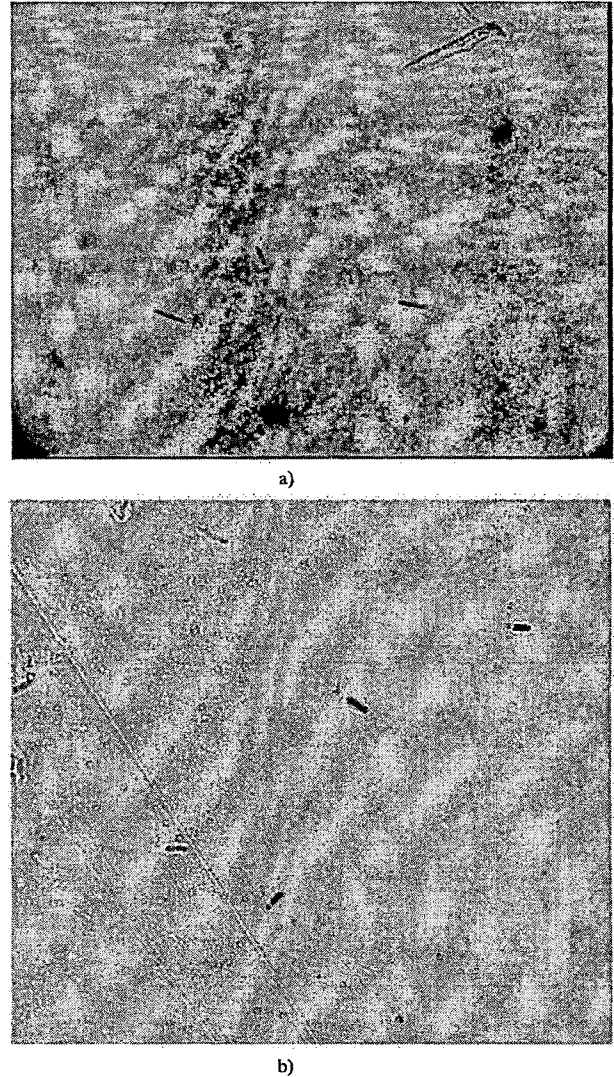
Fig. 2. (a), (b) Fission tracks of ca. 15 \mu\text{m} size with elliptical shapes from ^{233}\text{Pa}(2n_{\text{th}}, f) , recorded and developed on the Lexan detector with 500 \times magnification. Panels (a) and (b) correspond to different areas of the same slide and the image was taken with different microscopes using the same magnification. The size of the magnified view of the track area of the Lexan detector shown in (a) and (b) is 0.00159 \text{ cm}^2 .
