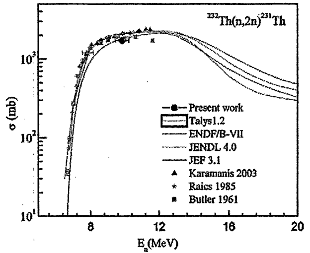
Fig. 8. (Colour on-line) Plot of the experimental and evaluated ^{232}\text{Th}(n, 2n) reaction cross-section as a function of the neutron energy from 5 MeV to 20 MeV. Experimental values from the present work and from refs. [36–44] are in different symbols, whereas the evaluated and theoretical values from TALYS are in solid lines with different colors.
