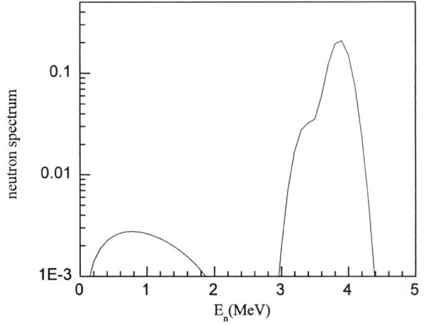
Fig. 5. Neutron spectrum from the ^7\text{Li}(p, n) reaction at E_p = 5.6 \text{ MeV} calculated using the results of Meadows and Smith of ref. [47].
