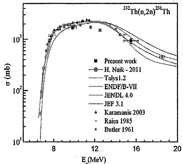
Fig. 5. Plot of the experimental and evaluated ^{232}\text{Th}(n, 2n) reaction cross-section as a function of the neutron energy from threshold to 20 MeV. Experimental values from present work and from refs. [33–35] are in different symbols, whereas the evaluated and theoretical values from TALYS are in solid lines with different colors.
