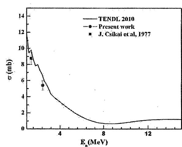
Fig. 3. Plot of experimental and evaluated ^{94}\text{Zr}(n, \gamma)^{95}\text{Zr} reaction cross section as a function of neutron energy of 1 to 15 MeV. Experimental values from the present work and from Ref. 23 are in different symbols and colors (color online); black solid line indicates the evaluated values from TENDL-2010.
