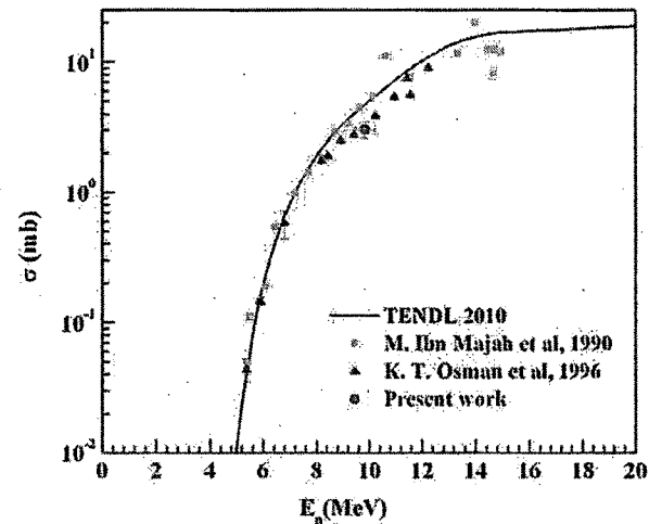
Fig. 4. Plot of experimental and evaluated ^{90}\text{Zr}(n, \gamma)^{90}\text{Y}^m reaction cross section as a function of neutron energy of 2 to 20 MeV. Experimental values from the present work and from Refs. 24 and 25 are in different symbols and colors (color online); black solid line indicates the evaluated values from TENDL-2010.
